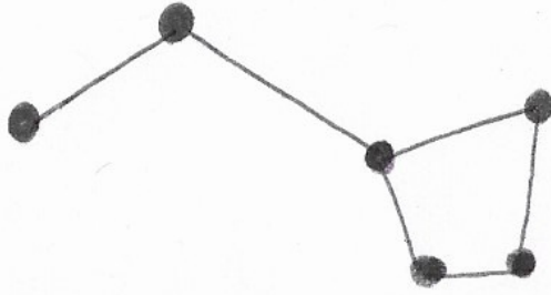
Osa Mayor
