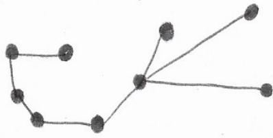
Scorpion
