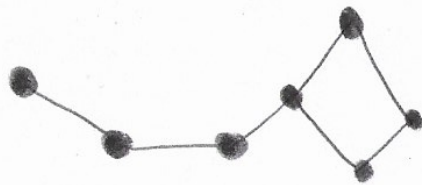
Ophiuchus
