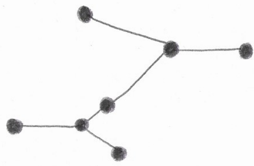
Can Major
